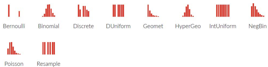
Figure 46: Common discrete distributions (Palisade @Risk)
