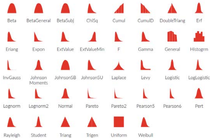
Figure 45: Common continuous distributions (Palisade @Risk)
